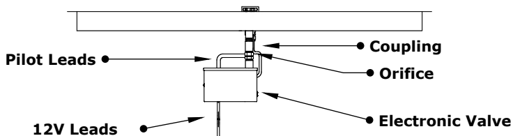
FRONT SIDE VIEW
