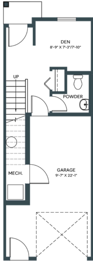
LOWER/ENTRY Lower Floor: 195 sq/ft
