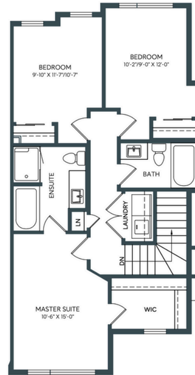
UPPER FLOOR
