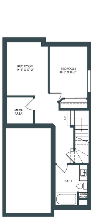
LOWER FLOOR
