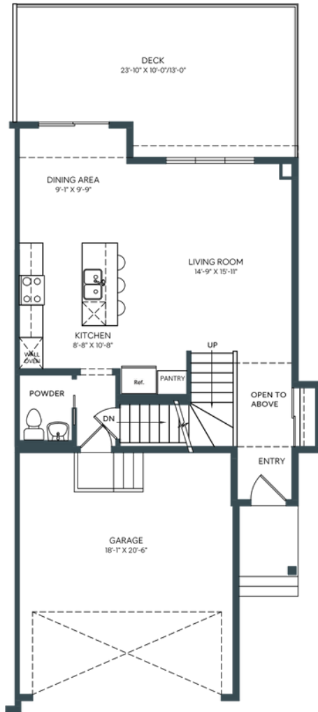
MAIN DOUBLE CAR GARAGE 668 sq/ft
