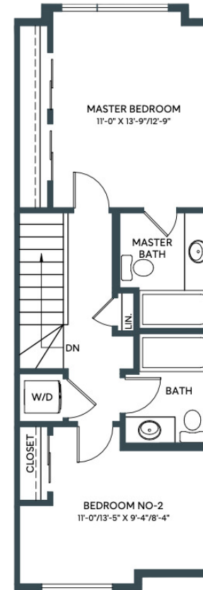
MAIN Second Floor: 563 sq/ft
