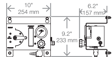
System Manifold - profile
