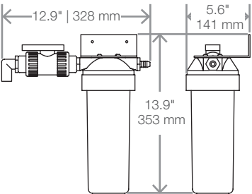
Pre-Filter Assembly
