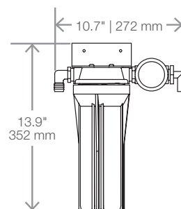
Pre-Filter
