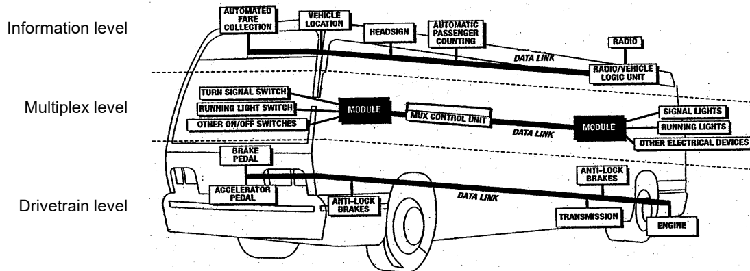
Data Communications Systems Levels
